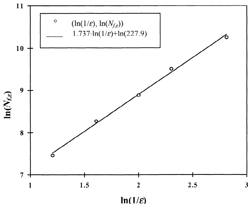
Figure 5. Dependence of \ln(N_{f,\varepsilon}) on \ln(1/\varepsilon) . The points (\ln(1/\varepsilon), \ln(N_{f,\varepsilon})) are distributed along the linear function with respect to \ln(1/\varepsilon) : 1.737 \ln(1/\varepsilon) + \ln(227.9) .
