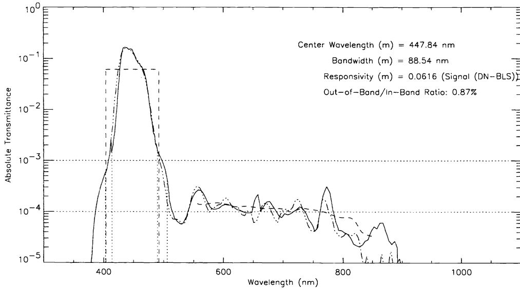
Figure 2. AirMISR measured spectral response profile for Band 1/ Blue.
