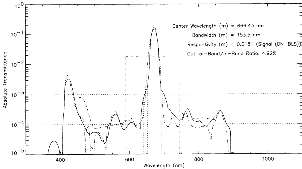
Figure 4. AirMISR measured spectral response profile for Band 3/ Red.
