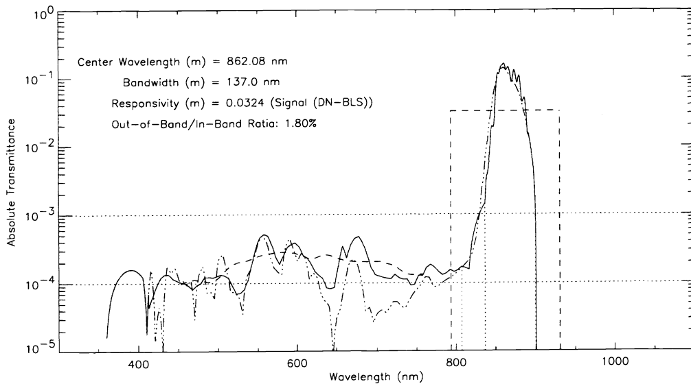
Figure 5. AirMISR measured spectral response profile for Band 4/ Near-infrared.
