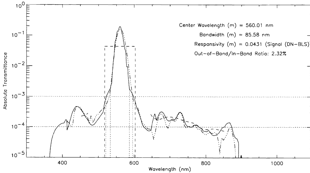
Figure 3. AirMISR measured spectral response profile for Band 2/ Green.
