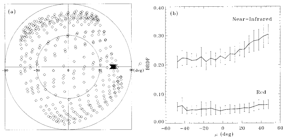
Fig. 1. Angular variation of the BRDFs of a homogeneous patch of needle leaf forest as measured by POLDER in June 1997 (55.36°N, 92.20°W) and the corresponding sun-view geometries. The symbols \diamond and \downarrow denote view and sun directions. The horizontal axis in panel (b) is expressed in terms \sin^{-1} \mu , where parameter \mu is defined in Fig. 6.
