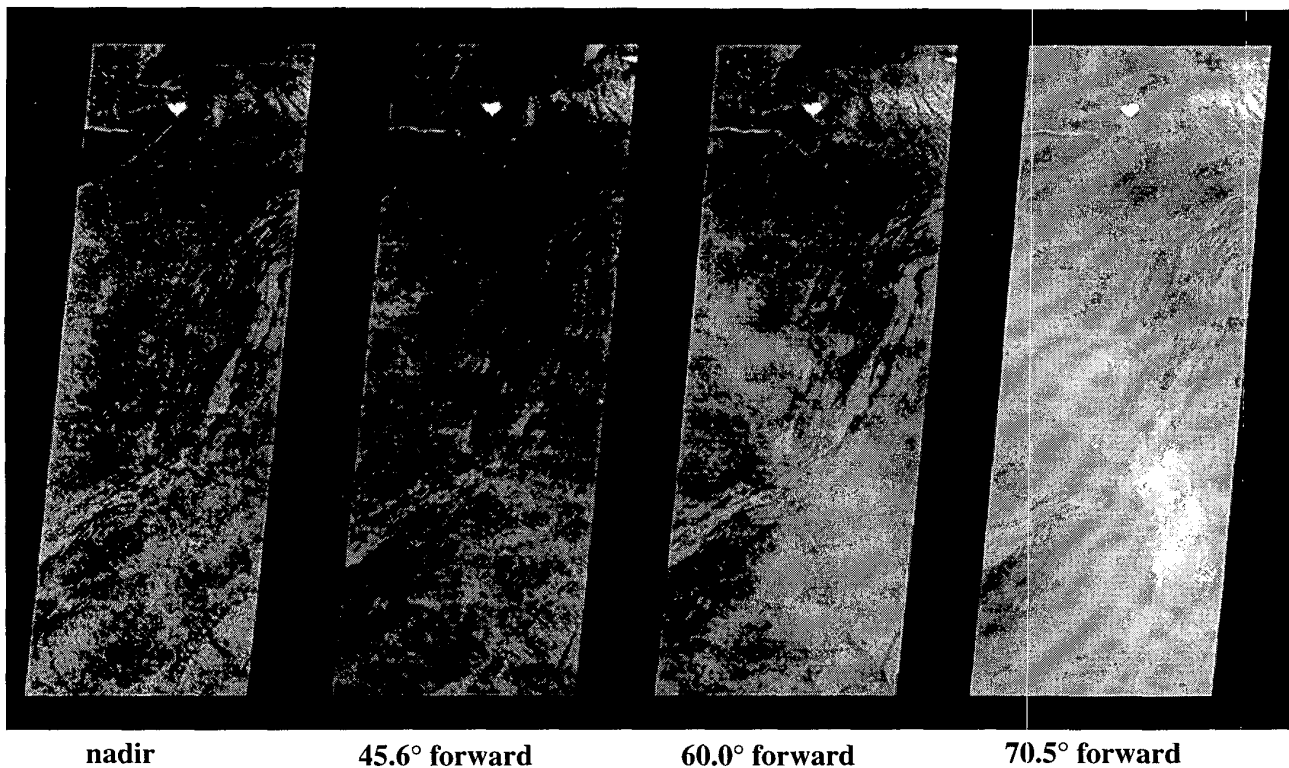
Figure 2. Multi-angle imagery obtained on March 6, 2000 over the eastern United States, stretching from Lake Ontario to Georgia. As the slant angle increases, the line-of-sight through the atmosphere grows longer and a pall of haze over the Appalachian Mountains becomes progressively more apparent. The images have been reproduced using the same radiometric scale. North is toward the top.
