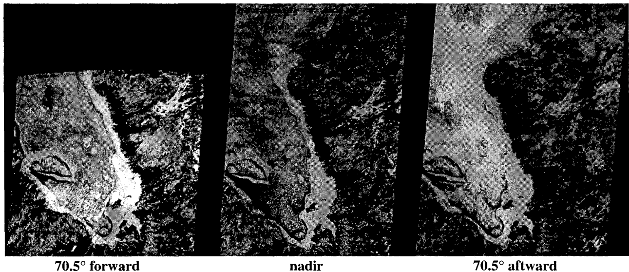
Figure 1. "First light" imagery obtained on February 24, 2000 over the ice-covered James Bay in the Ontario-Quebec region of Canada. The abrupt transition from dark to light in the left image marks the opening of MISR's cover as the forward camera was viewing this scene. The image acquired by the nadir camera was obtained about 3.5 minutes later, and the aftward image was acquired about 7 minutes after the forward view. Changes in brightness and contrast with angle distinguish different environmental conditions, notably the fast (smooth) ice, pack (rough) ice, and clouds. North is toward the top.
